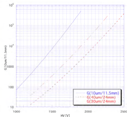
Fig. 2 : Gas gain
