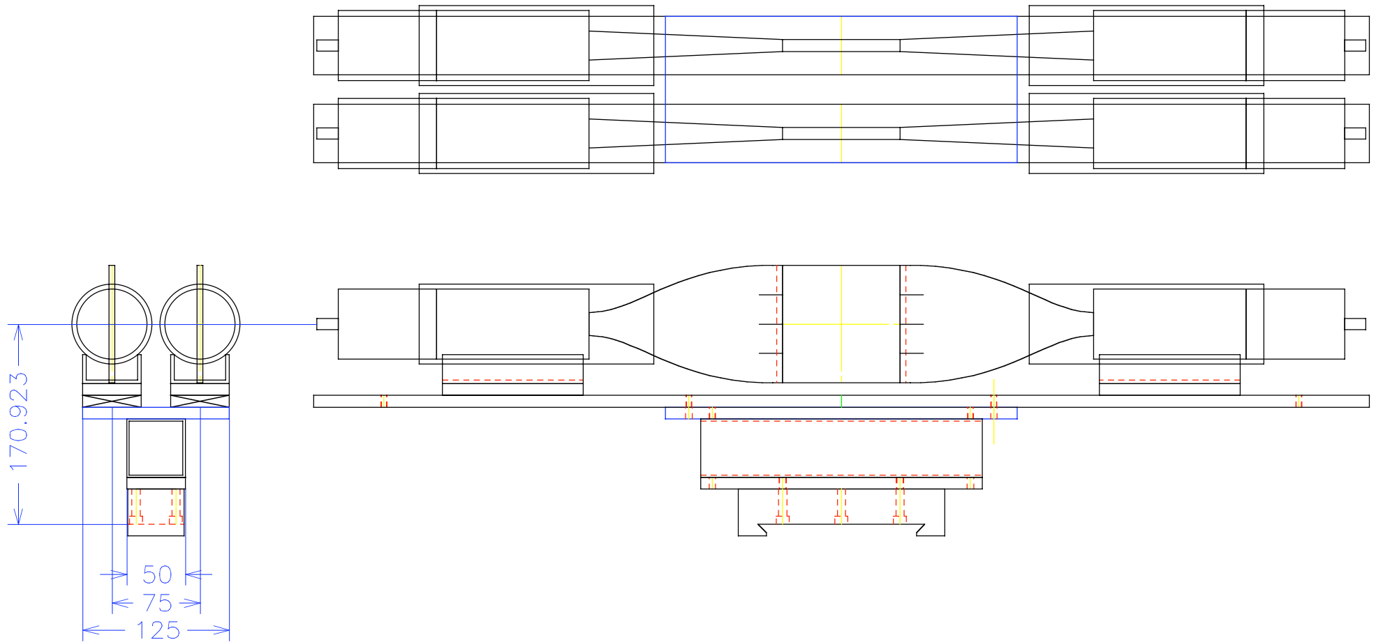
SF3-A/B Assembly for P224 1mmt plastic/R329/Tr-Base/MHV/1-Anode 23-Apr-2007 Kobayashi T.
